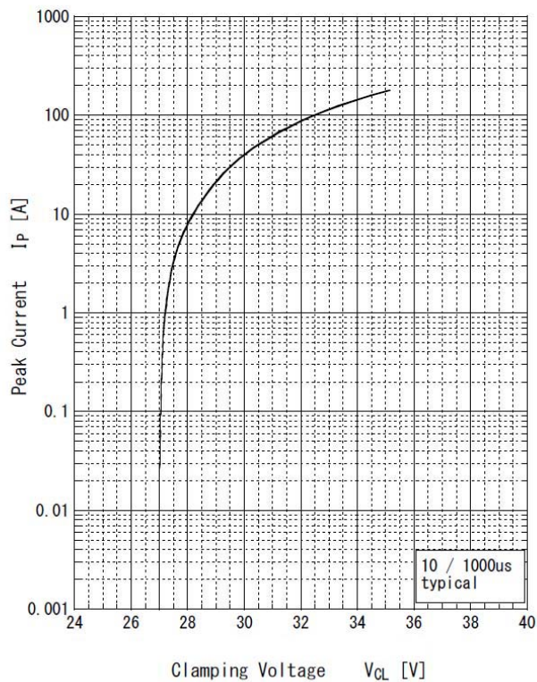
Clamping Voltage vs Peak Current
