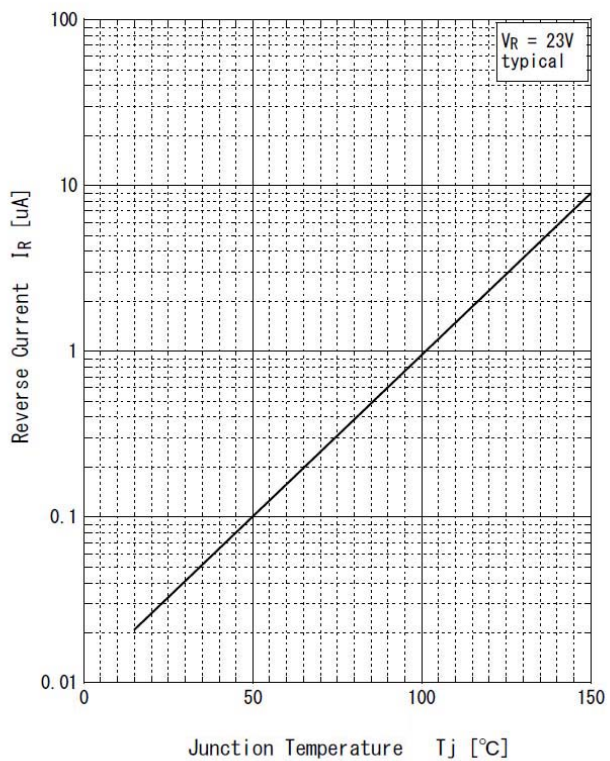
Reverse Current vs Junction Temperature
