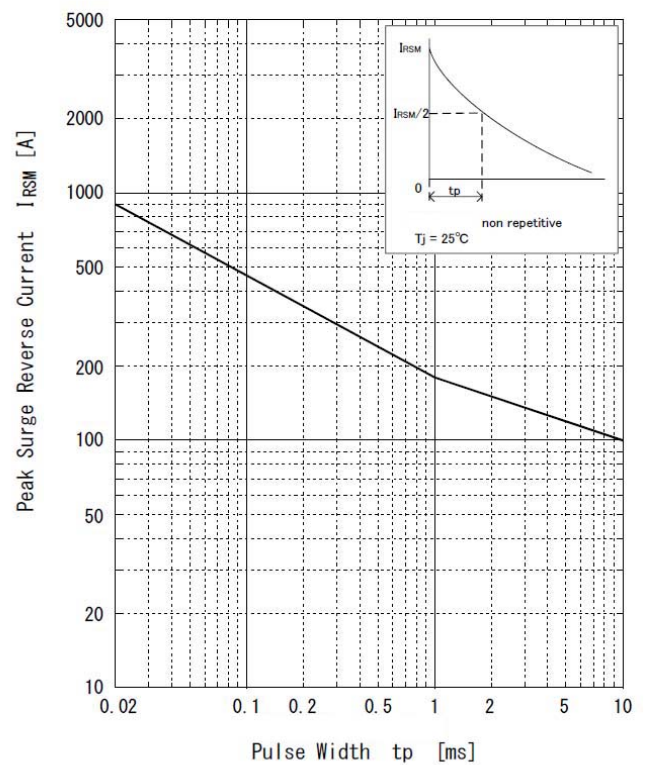
Peak Surge Reverse Current
