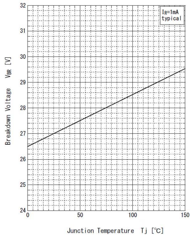
Breakdown Voltage vs Junction Temperature
