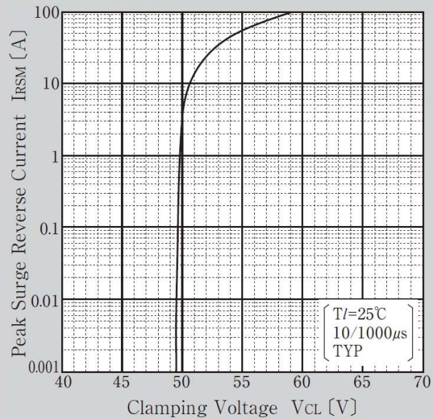
Clamping Voltage
