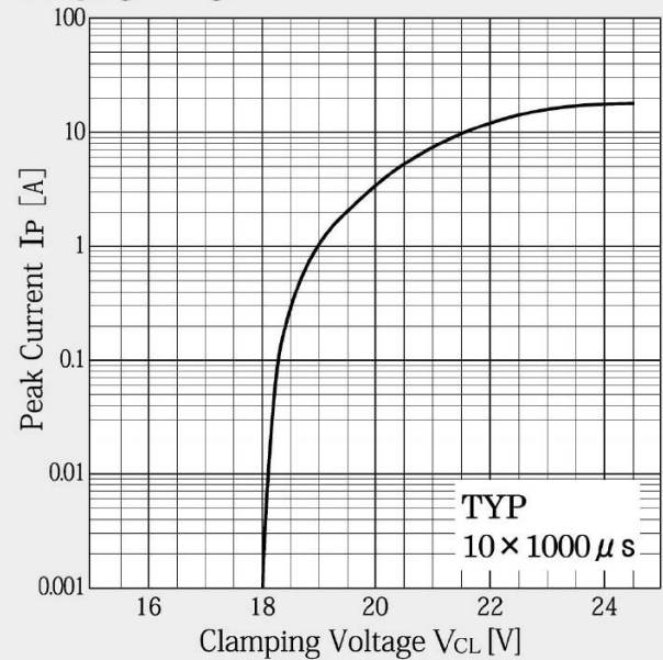
Clamping Voltage
