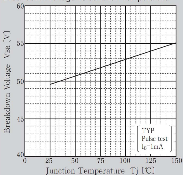
Breakdown Voltage vs Junction Temperature
