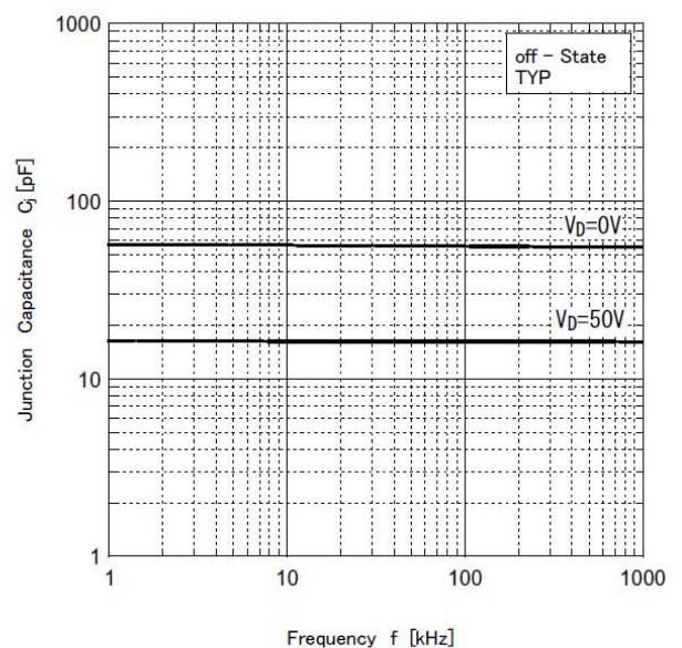
Junction Capacitance
