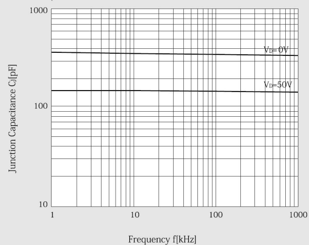
Junction Capacitance
