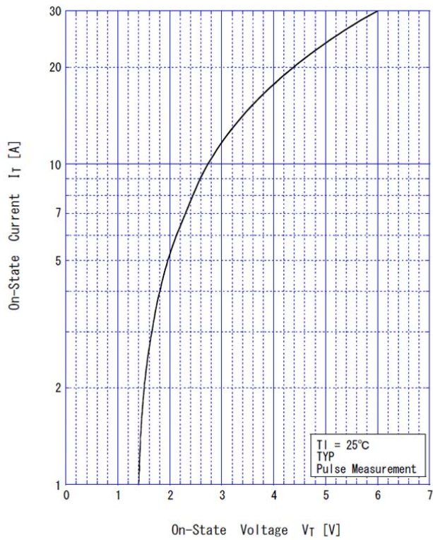
On-State Voltage vs On-State Current
