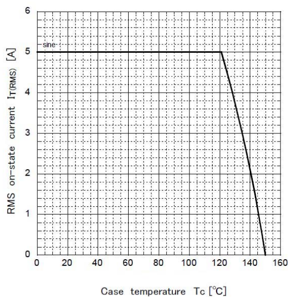
Derating curve T_c - I_{T(RMS)}
