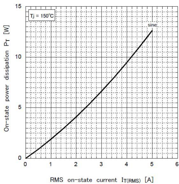
On-state power dissipation
