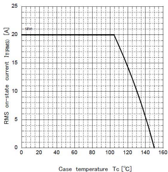
Derating curve T_c - I_T(\text{RMS})
