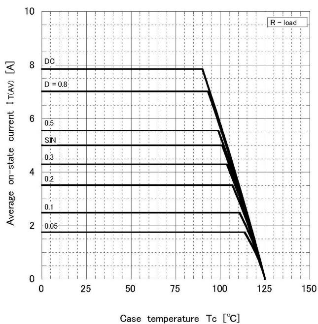
Average on-state current vs Case temperature
