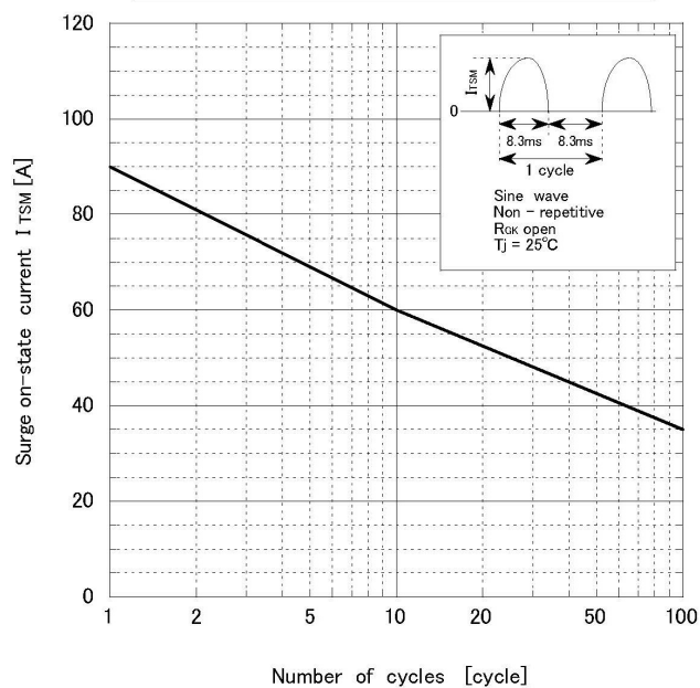
Surge on-state current vs Number of cycles
