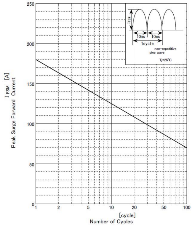
SG15SC6M Peak Surge Forward Capability
