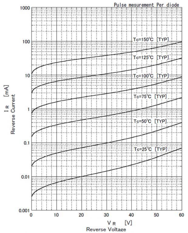
SG15SC6M Reverse Current
