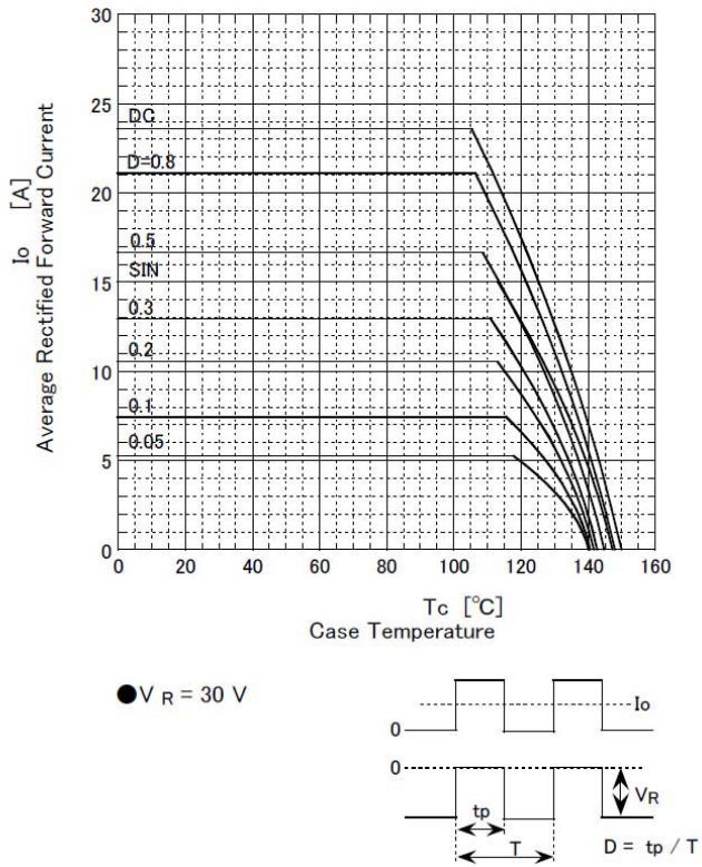
Derating Curve
