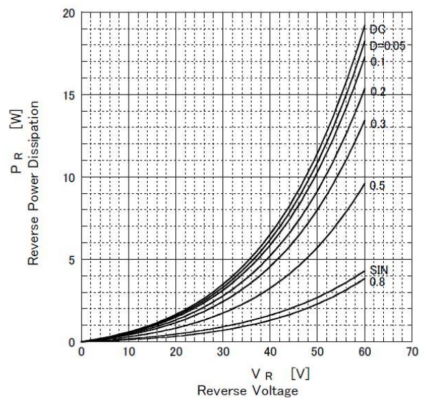
SG15SC6M Reverse Power Dissipation
