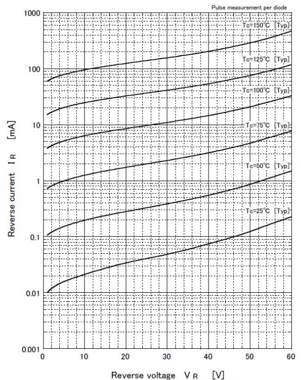
Reverse current
