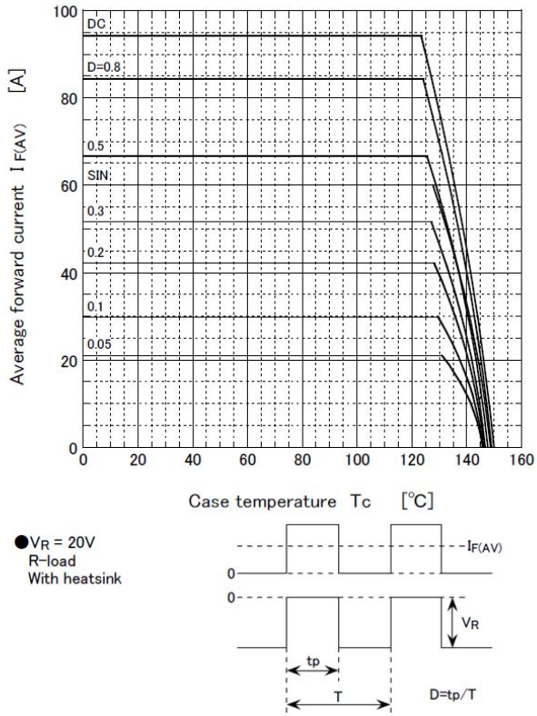
Derating curve
