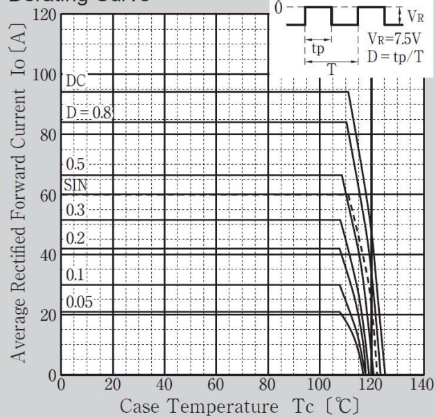
Derating Curve
