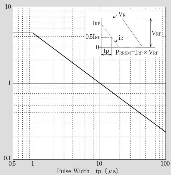
Repetitive Surge Reverse Power Capability
