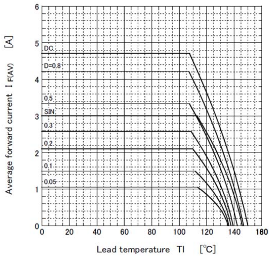
Derating curve
