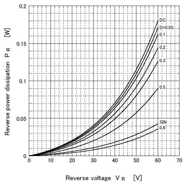
Reverse power dissipation
