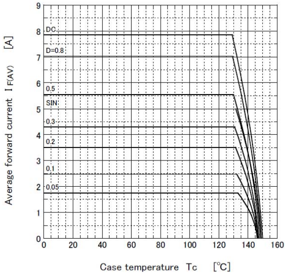
Derating curve
