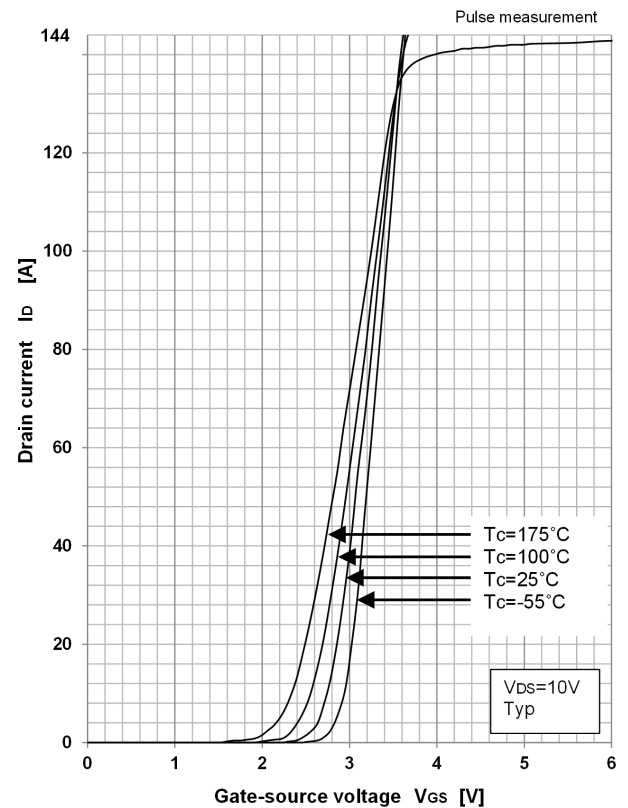
Transfer characteristics
