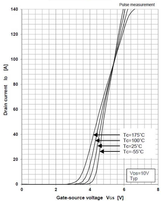
Transfer characteristics
