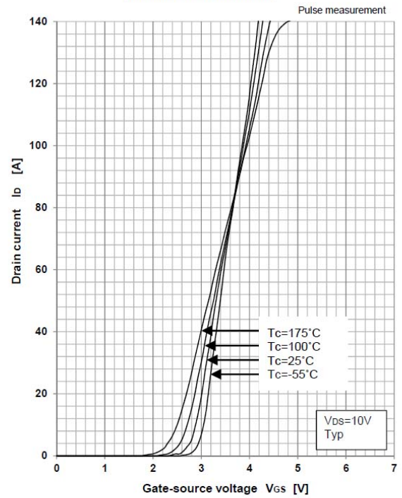
Transfer characteristics
