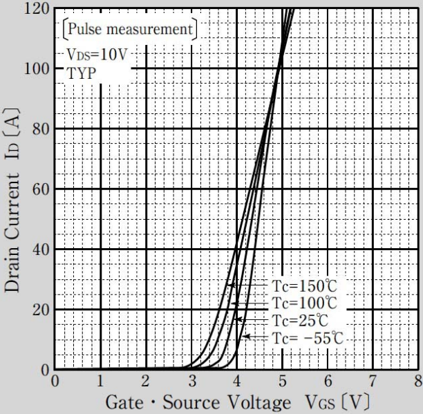
Transfer Characteristics
