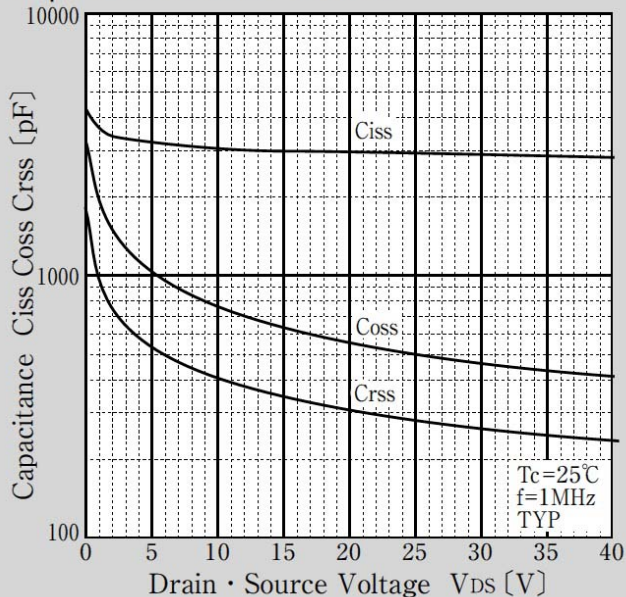
Capacitance Characteristics
