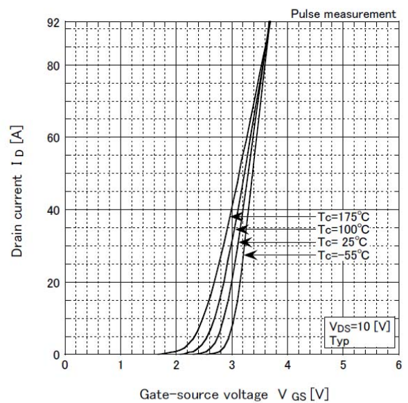
Transfer characteristics
