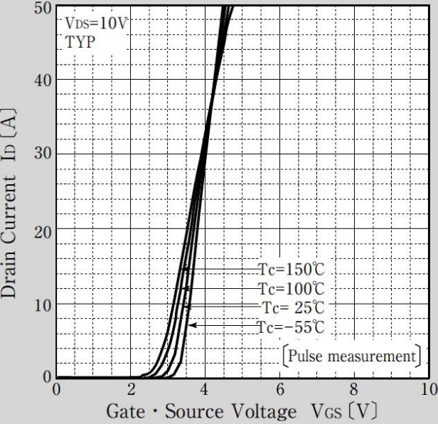
Transfer Characteristics
