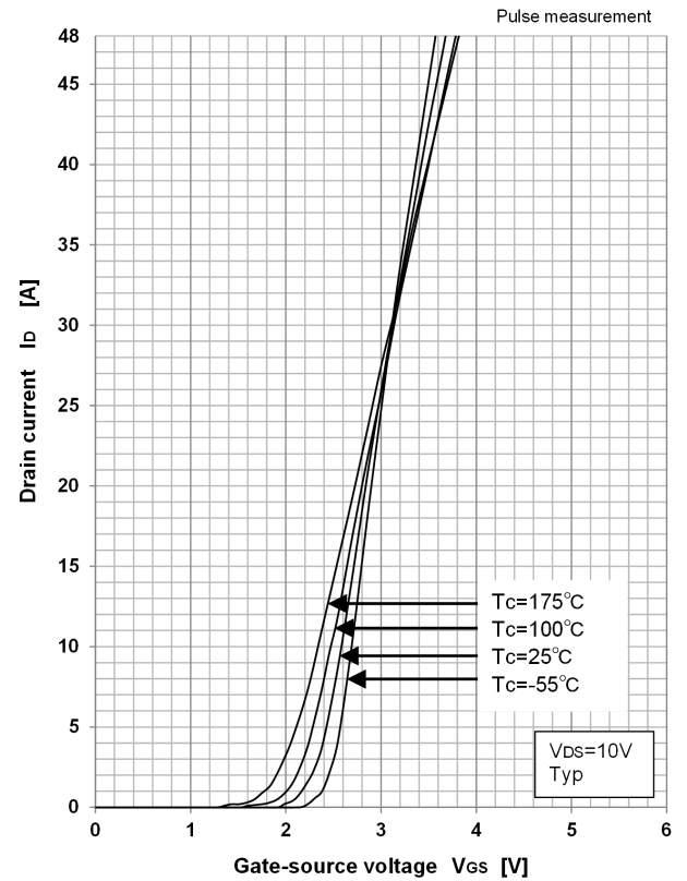
Transfer characteristics
