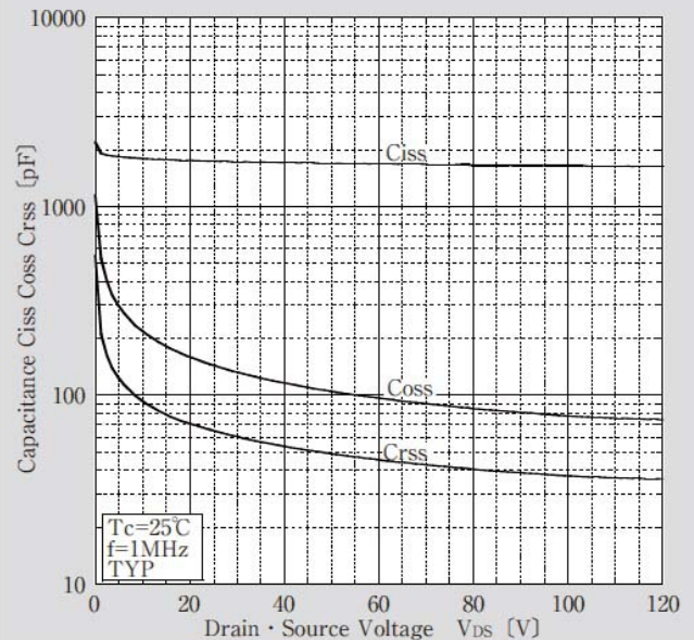
Capacitance Characteristics
