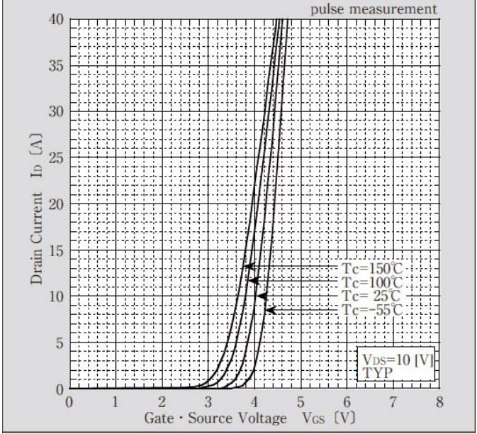
Transfer Characteristics
