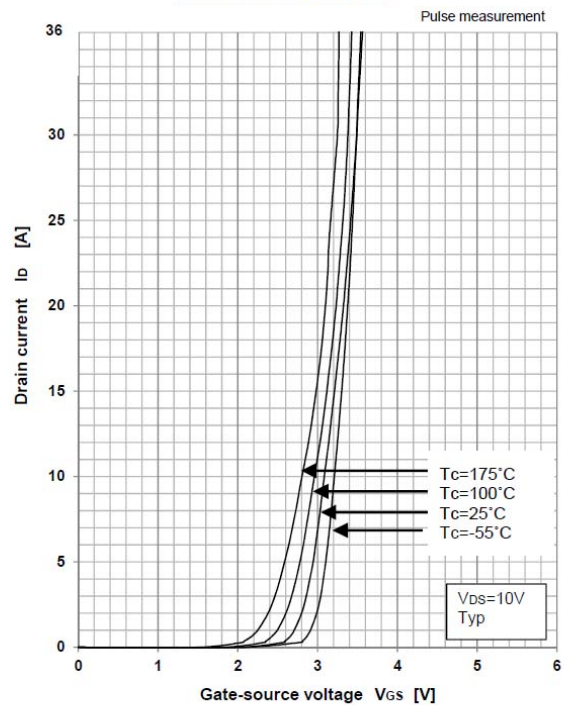
Transfer characteristics
