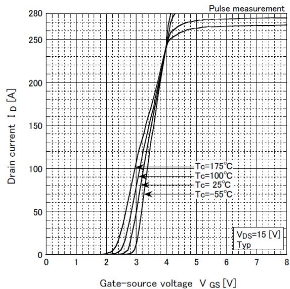
Transfer characteristics
