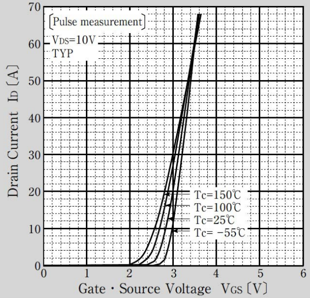
Transfer Characteristics
