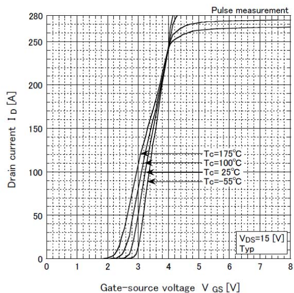
Transfer characteristics
