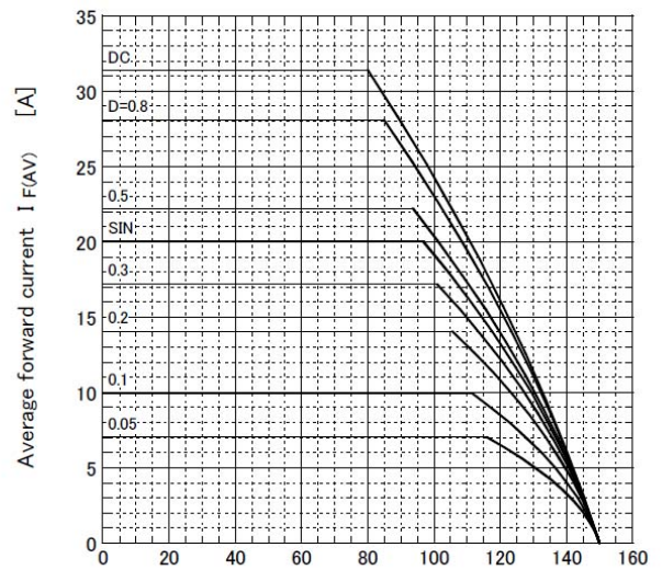
Derating curve
