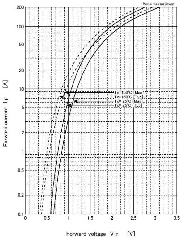
Forward voltage
