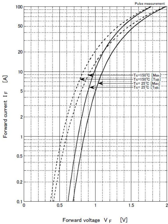
Forward voltage
