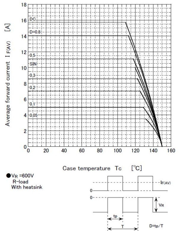
Derating curve
