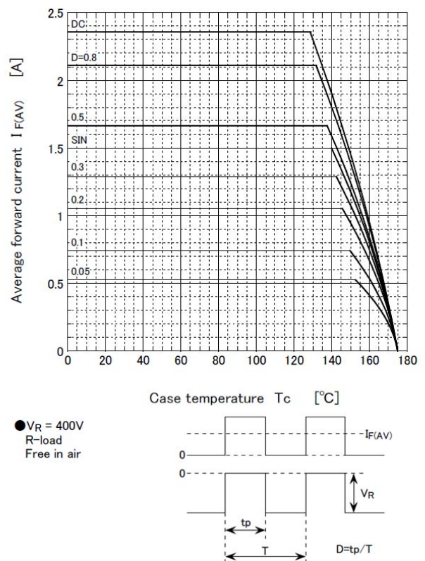
Derating curve
