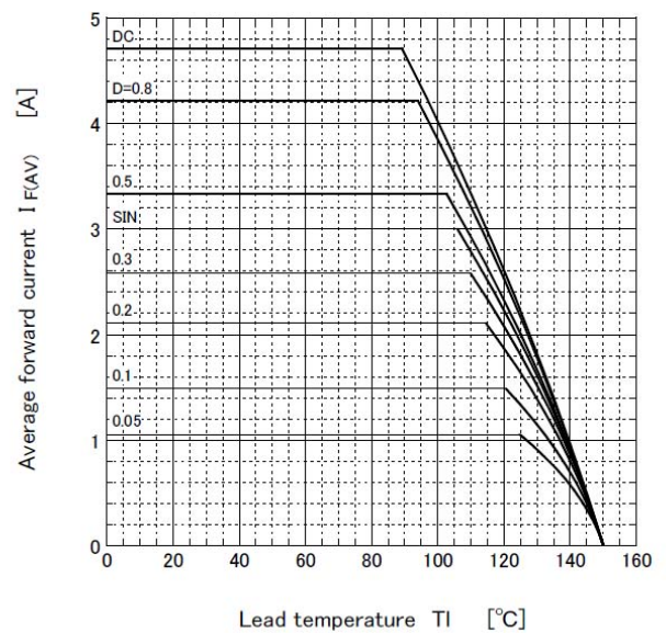
Derating curve
