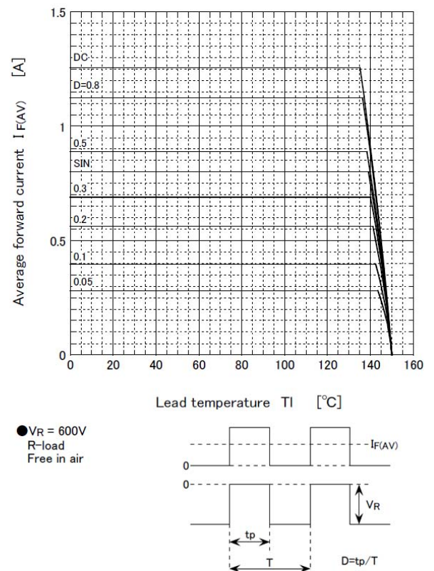
Derating curve
