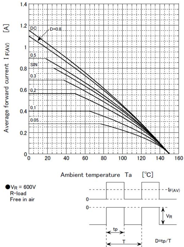
Derating curve
