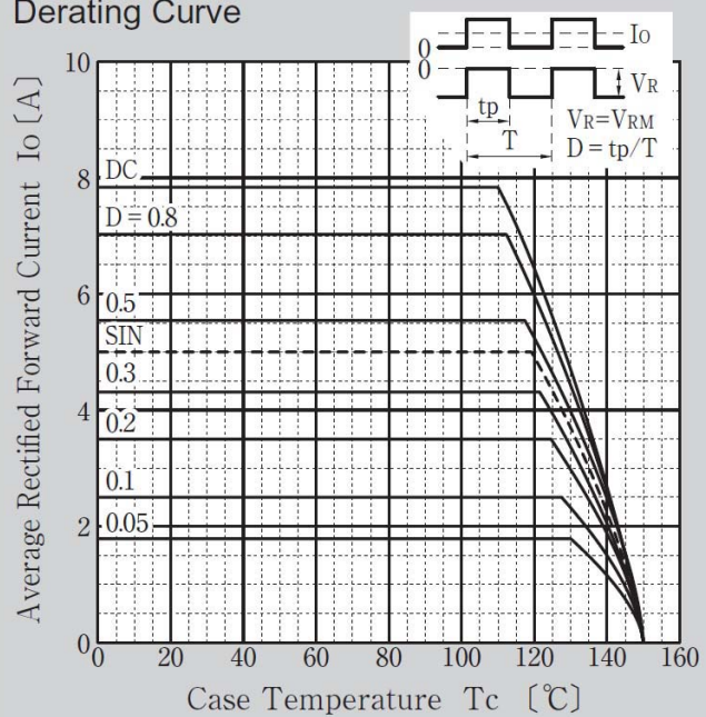
Derating Curve
