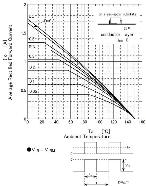
Derating Curve
