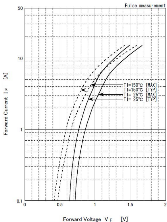
Forward Voltage
