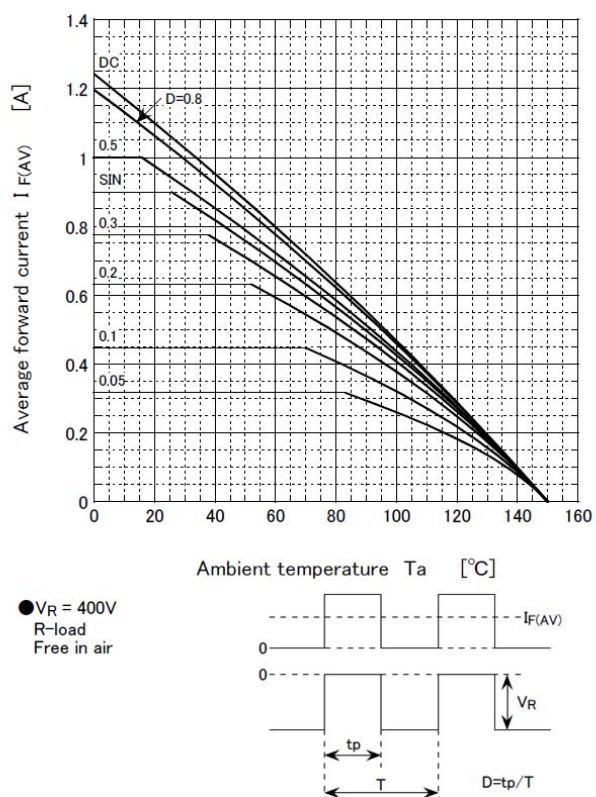
Derating curve
