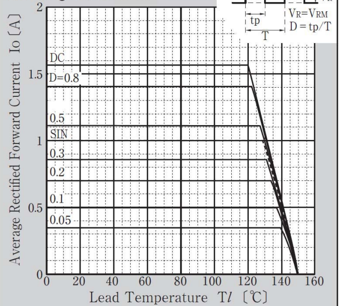
Derating Curve T_I - I_O
