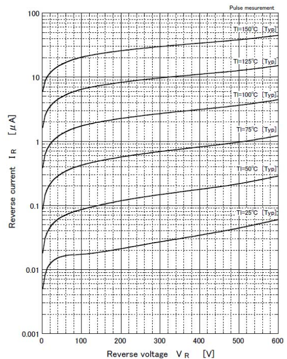
Reverse current
