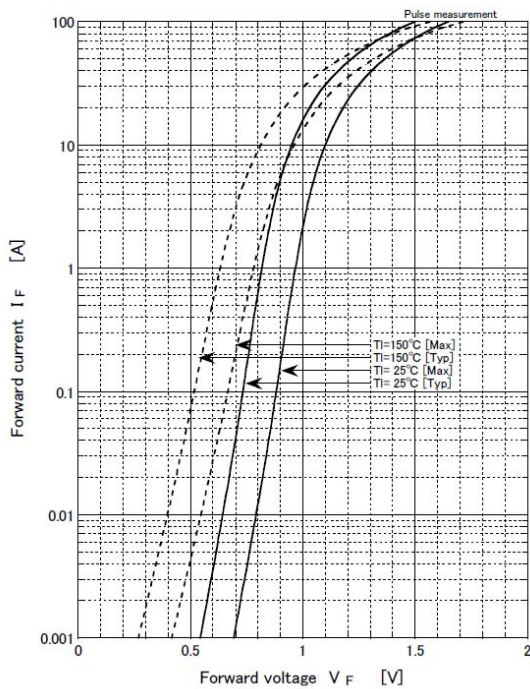
Forward voltage
