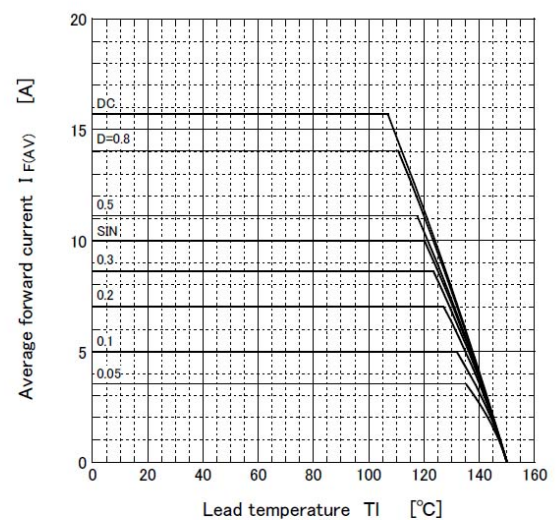
Derating curve
