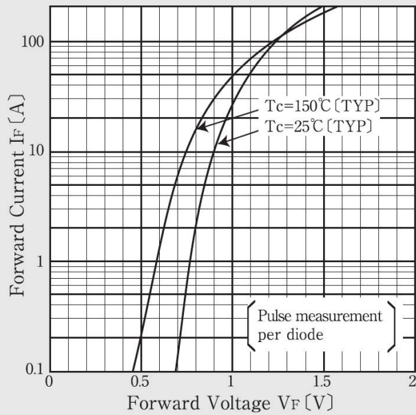
Forward Voltage
