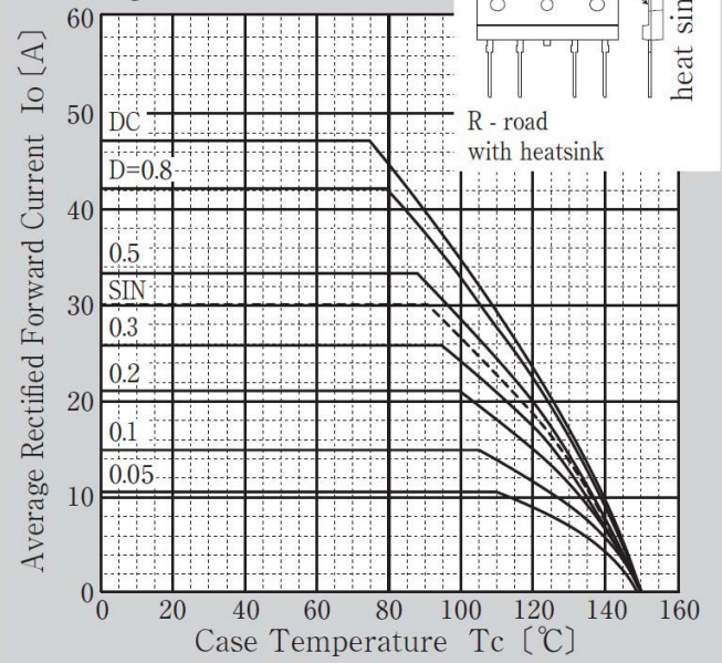
Derating Curve
