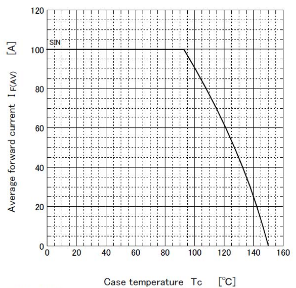
Derating curve
